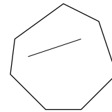
Convex polygon
