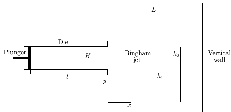
Fig. 4. Geometry of the two-dimensional cavity and initial position of the jet.
