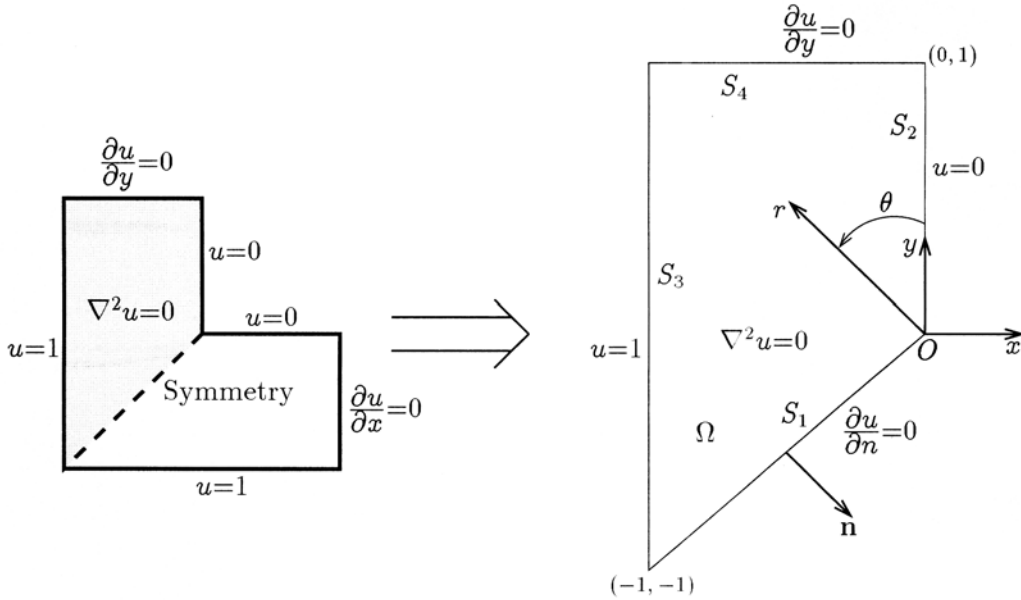
Figure 1. Geometry and boundary conditions of the test problem
